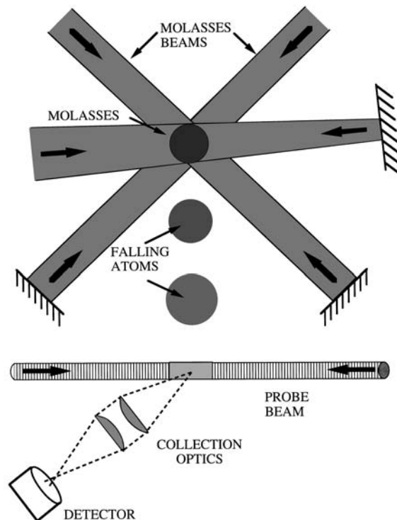
FIG. 15. Time-of-flight method for measuring laser cooling temperatures.
